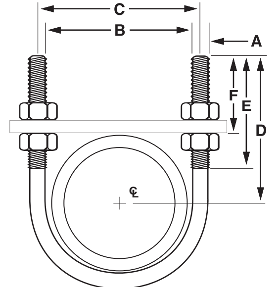
Figure 137 U-Bolt
